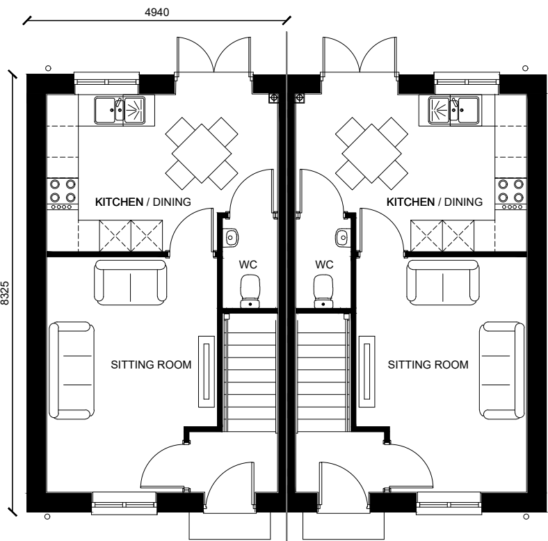
PROPOSED GROUND FLOOR PLAN AS OPP
