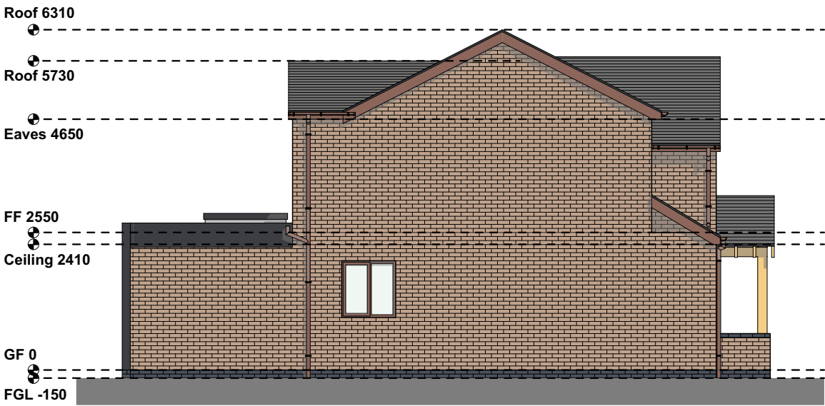
Side Elevation
