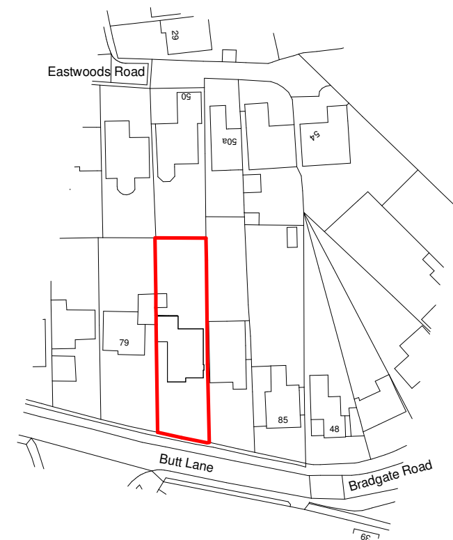
Location Plan 1:1250
