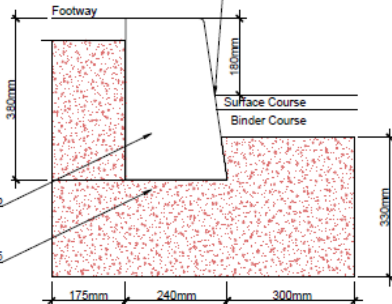
Bus Stop Kerb Detail BK1
