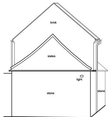
Existing East Elevation 1:100
