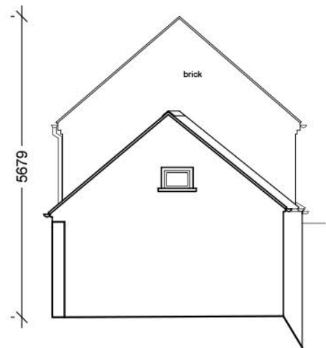
Existing West Elevation 1:100
