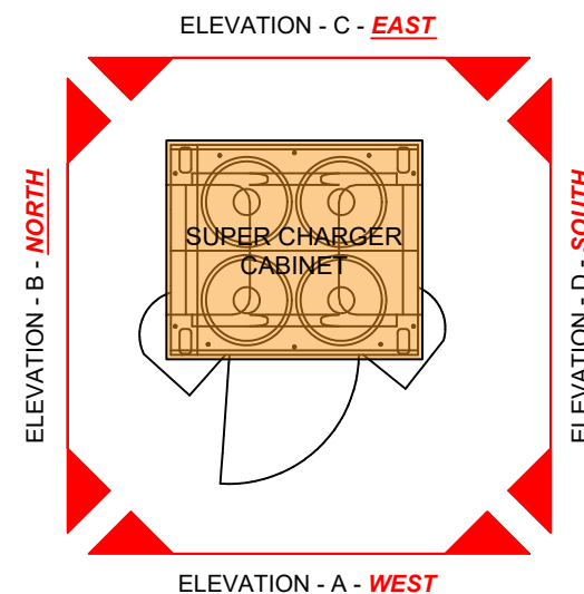
TESLA SUPPLY CABINET SCALE - 1:50
