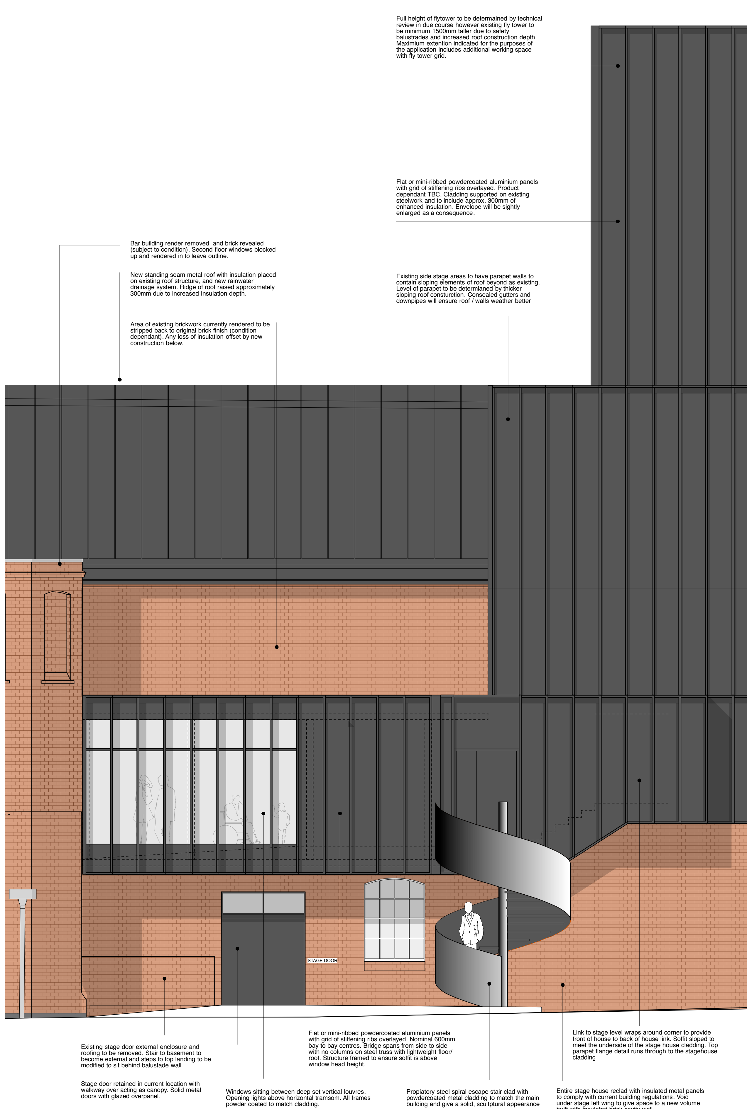
AMBULATORY DETAILED ELEVATION
