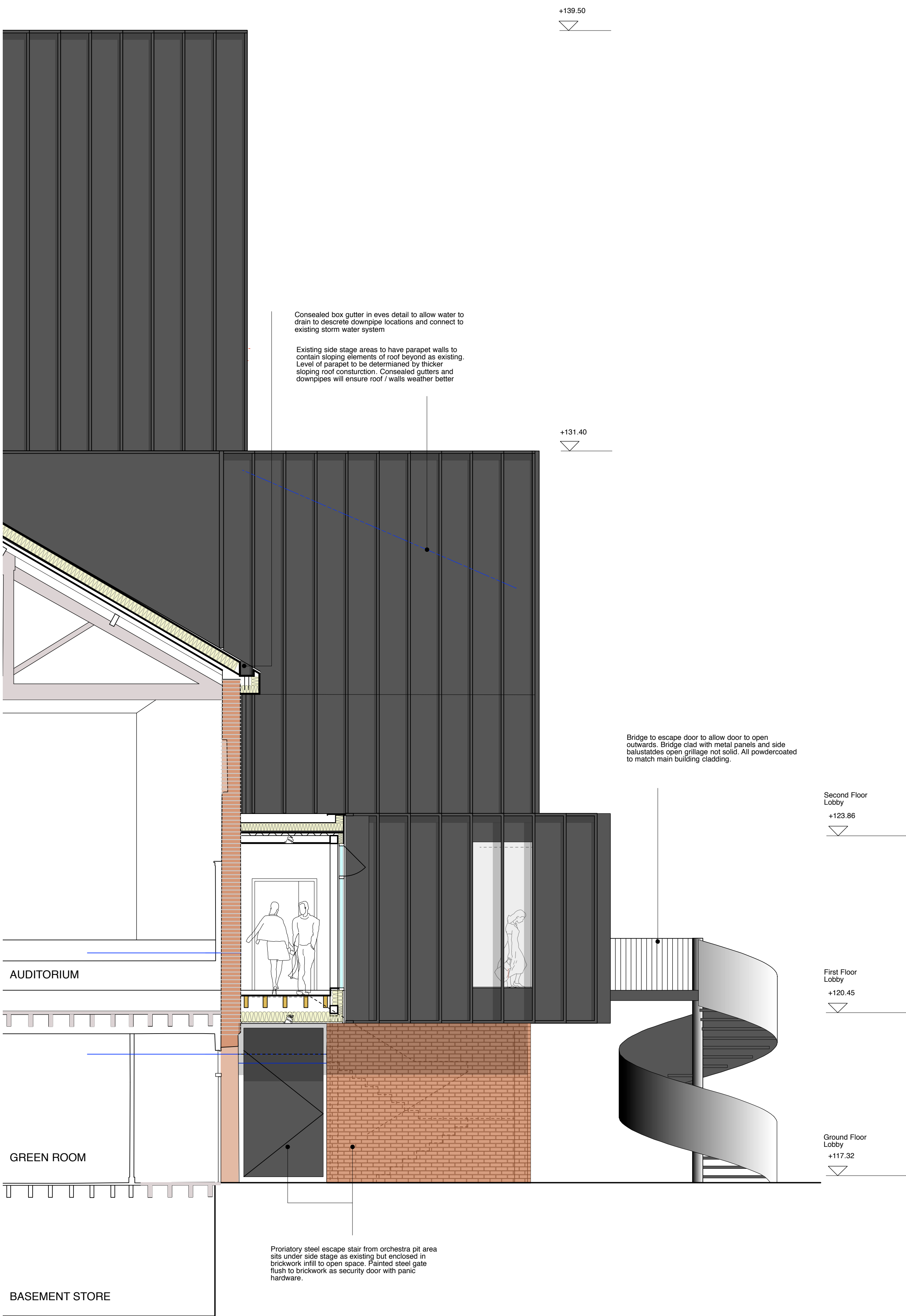
AMBULATORY DETAILED SECTION
