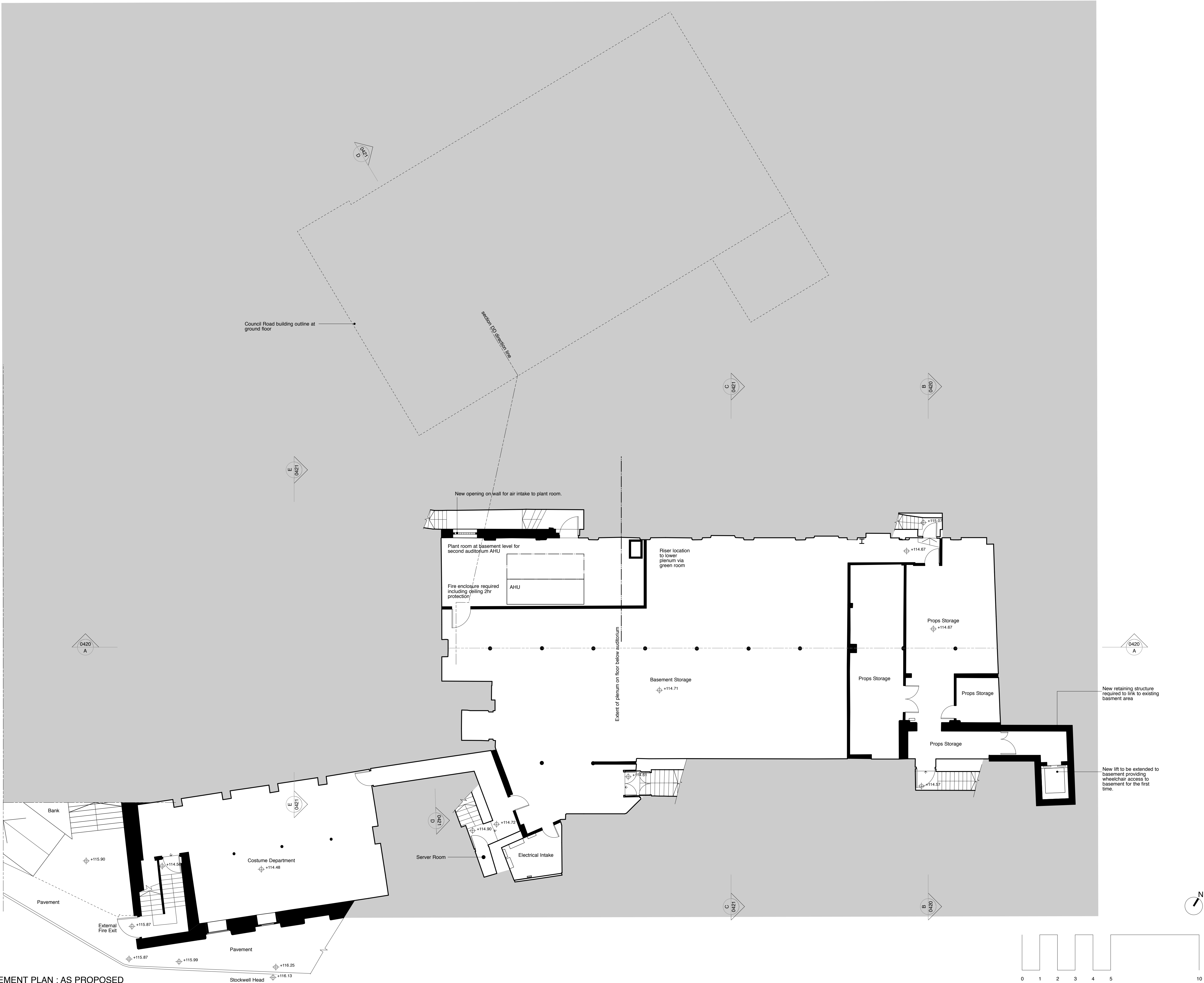
BASEMENT PLAN : AS PROPOSED
