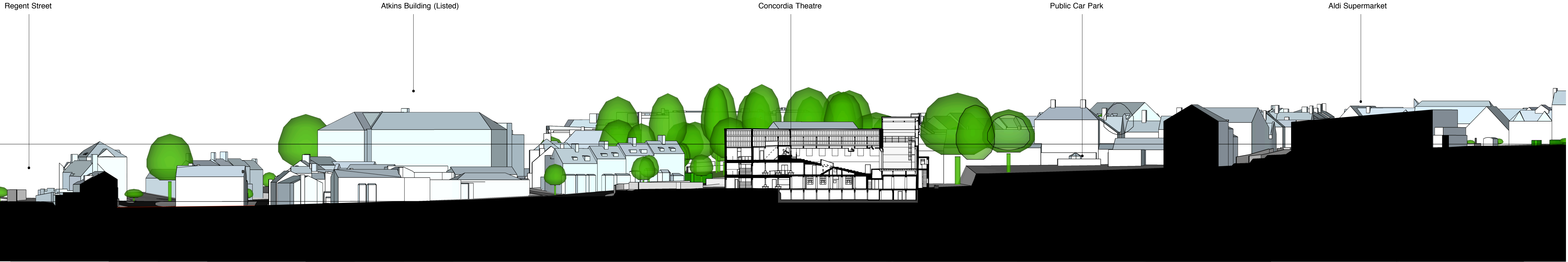
SECTION XX : AS EXISTING 1:500
