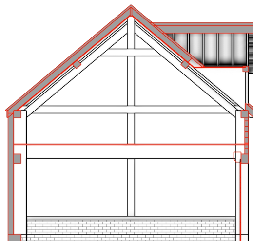
Dormer Cross section 1:100 @ A3
