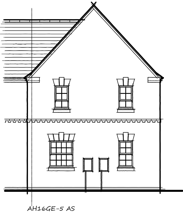
Side Elevation
