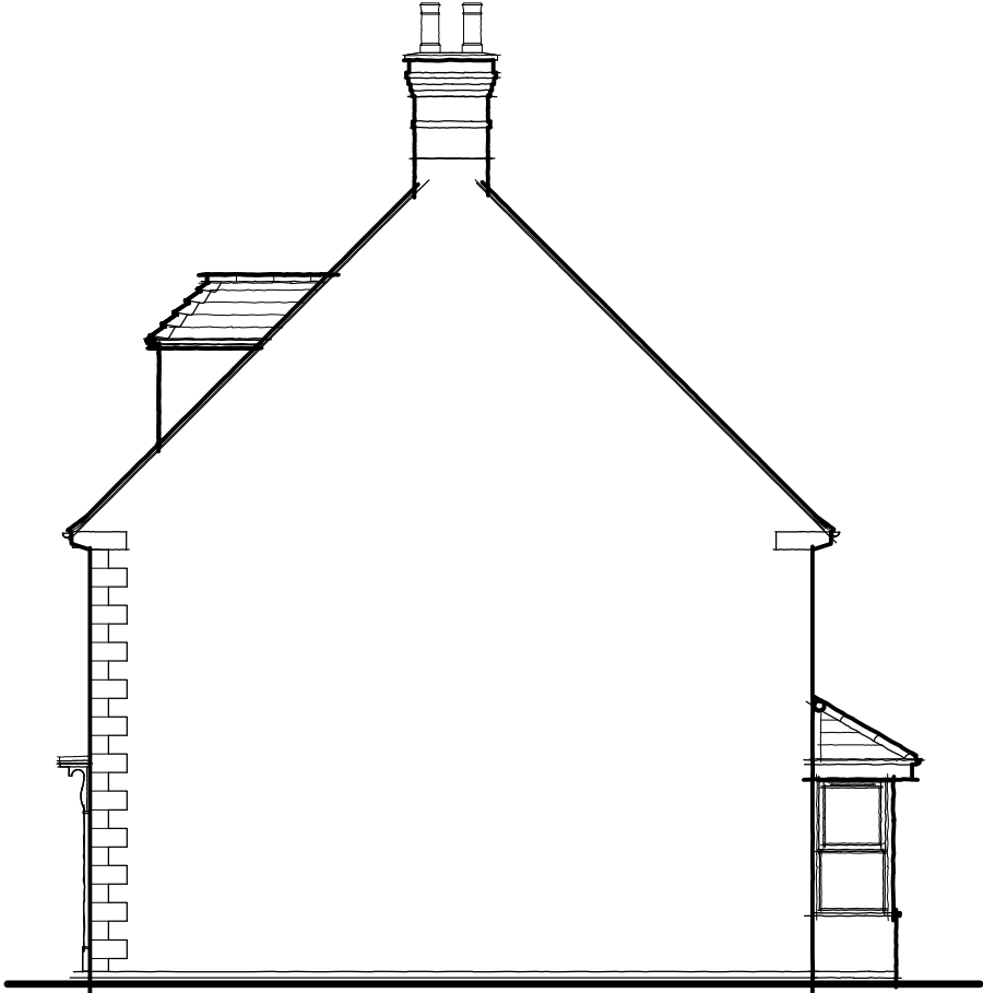
Side Elevation
