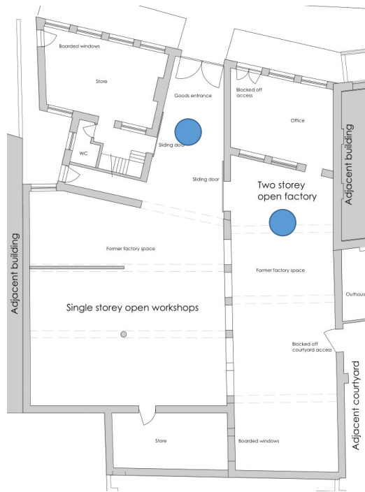
Ground Floor Plan Extract – see dwg 012
