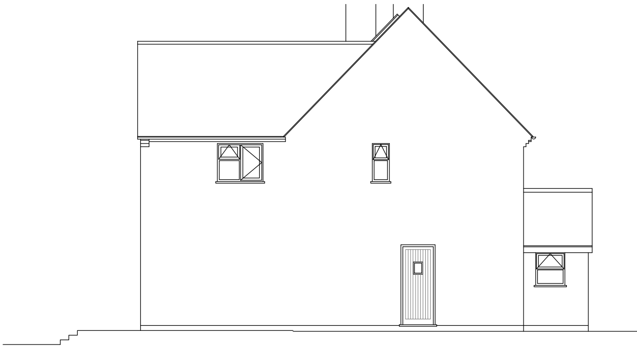
EXISTING / PROPOSED SIDE ELEVATION
