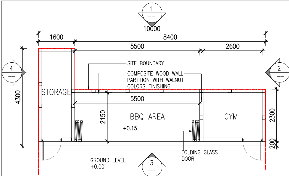
PROPOSED LAYOUT OF GARDEN HOUSE
