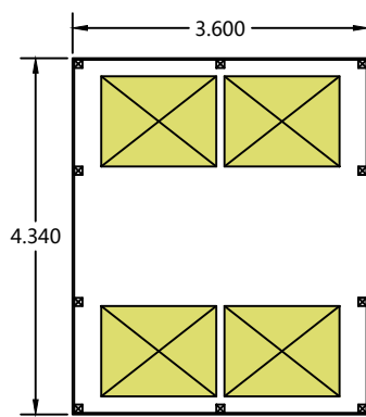
Bin Store 1:100
