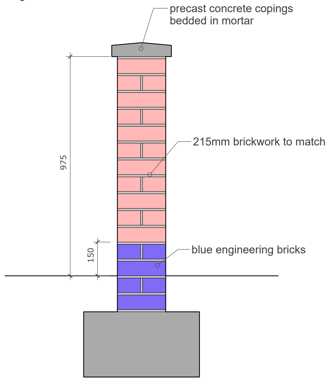
DETAIL OF NEW BOUNDARY WALL 1:10
