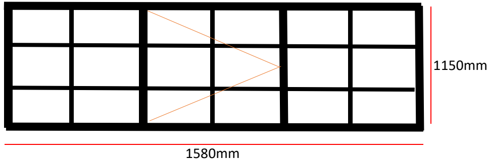
Bathroom Window
