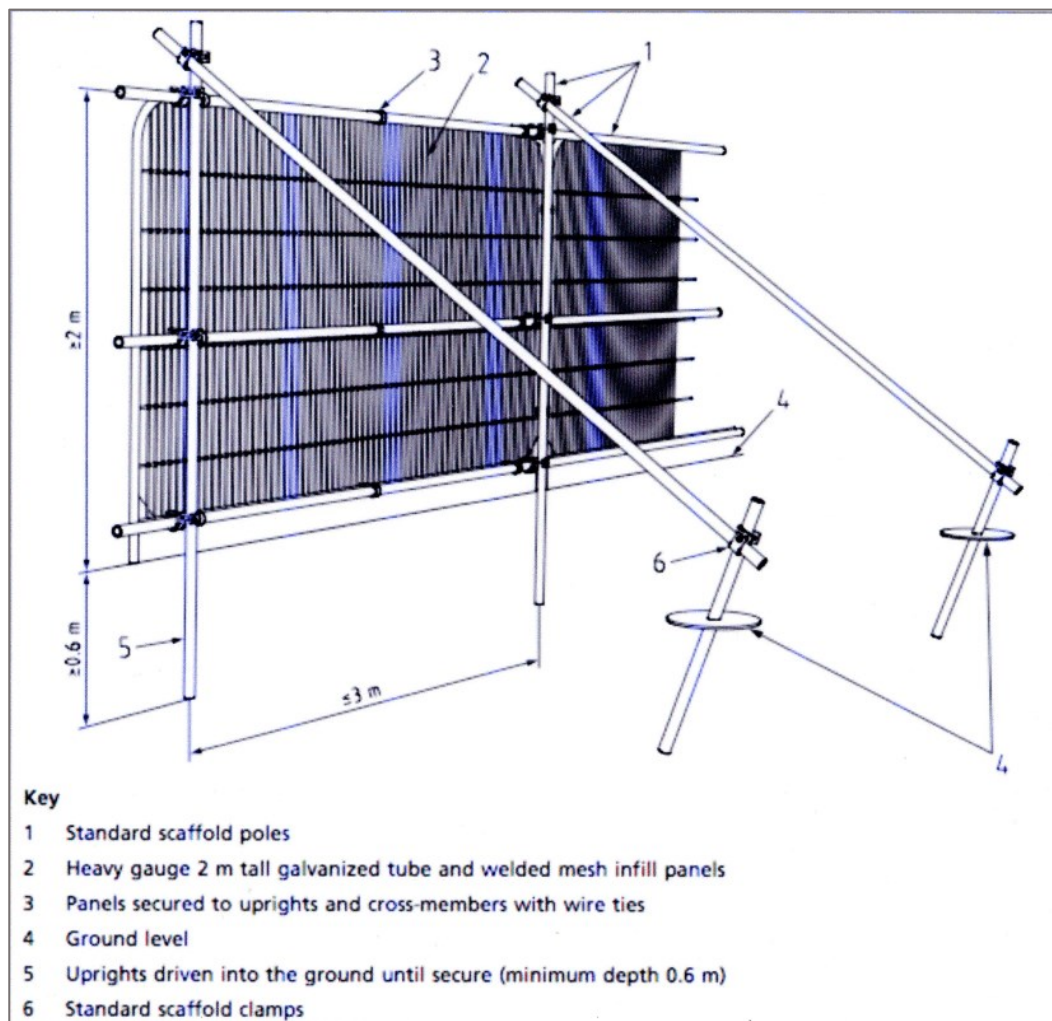
Figure 1: Default Specification for Protective Barrier (Tree Protection Fencing – TPF) (Taken from Figure 2 of Section 6 BS5837:2012)
