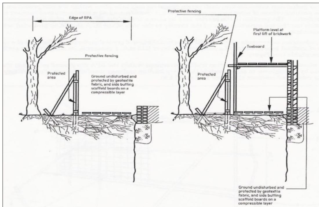
Figure 3: Default Specification for the installation of scaffolding within RPAs
