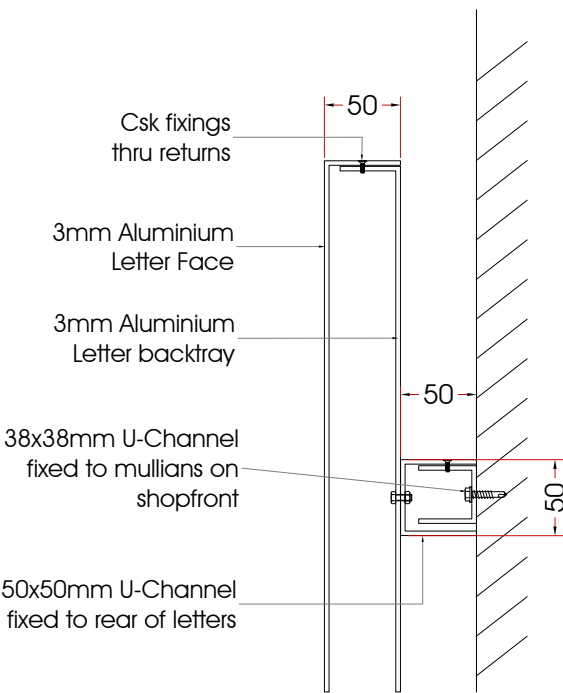
Sign 2 Section 1:5@A4
