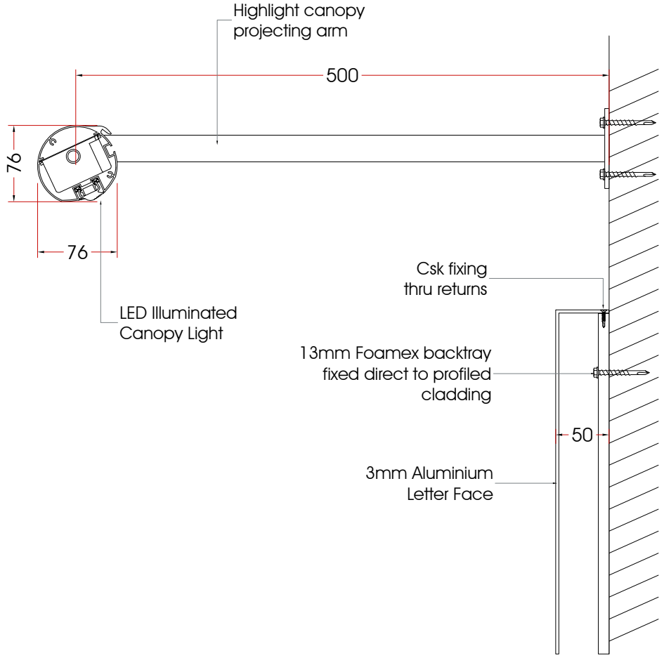
Sign 3 Section 1:5@A4
