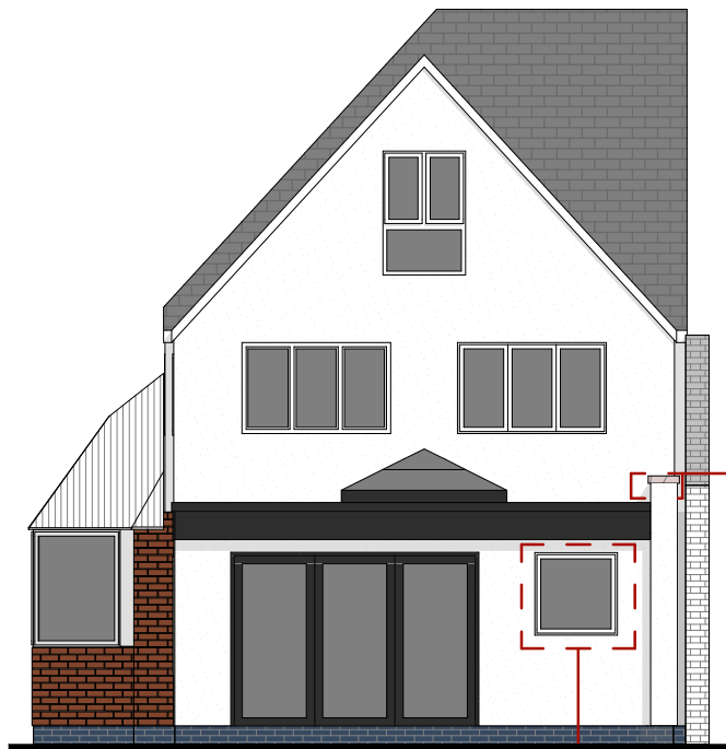
West Elevation - Rear
